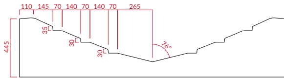
SECTION A
