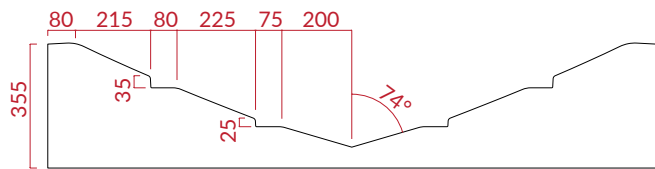
SECTION A
