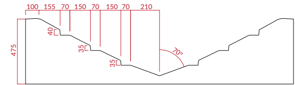
SECTION C
