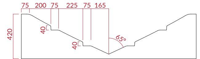
SECTION C
