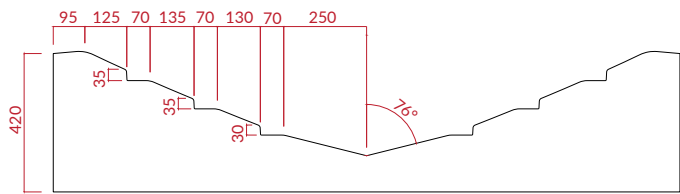
SECTION A
