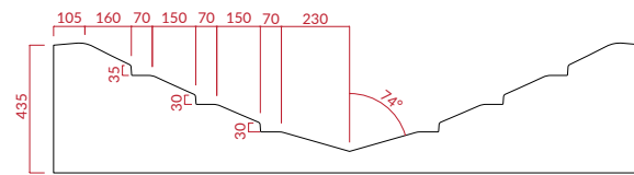
SECTION B
